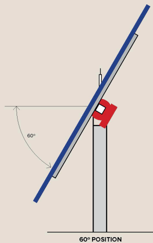
Work positions if WS < 77 km/h (+/- 60°)
